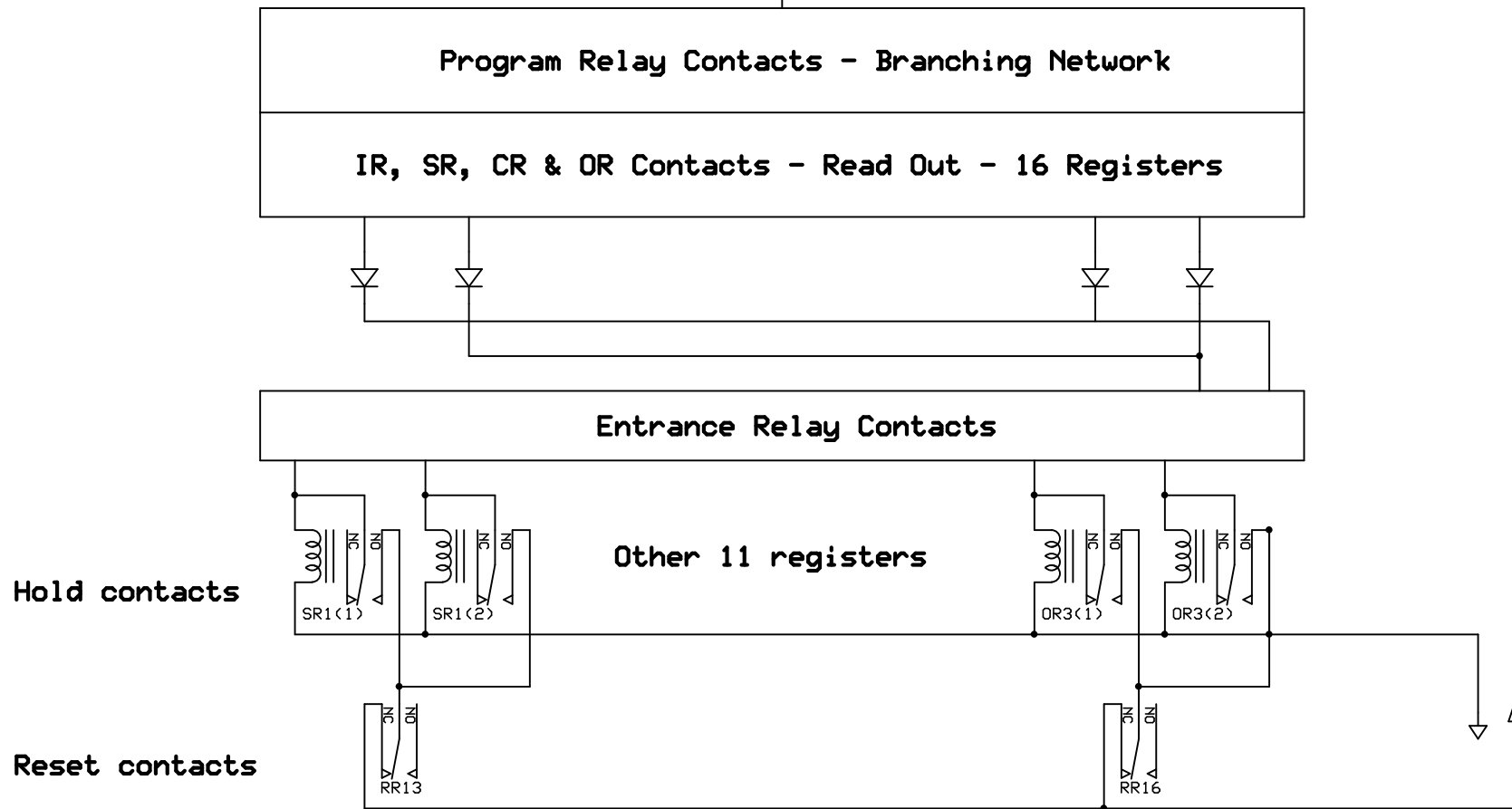
Circuit 9 - Select Sending Register and Transfer Circuit
